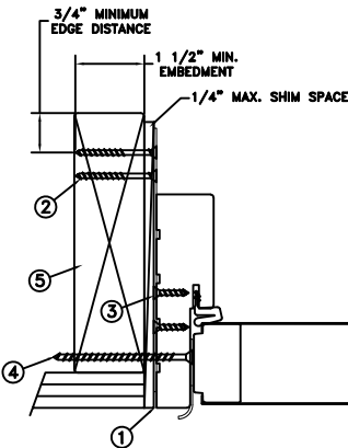
FRAME JAMB SECTION (TYP) HORIZONTAL SECTIONS
