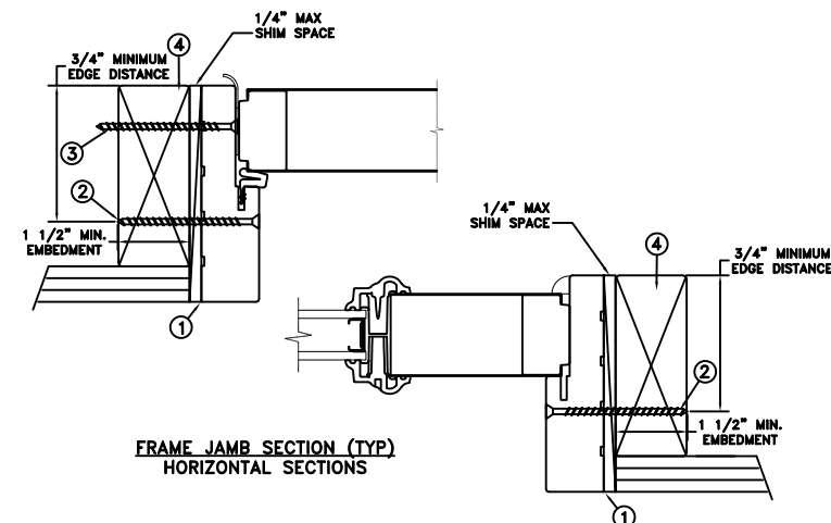
FRAME SECTION (TYP) VERTICAL SECTION
